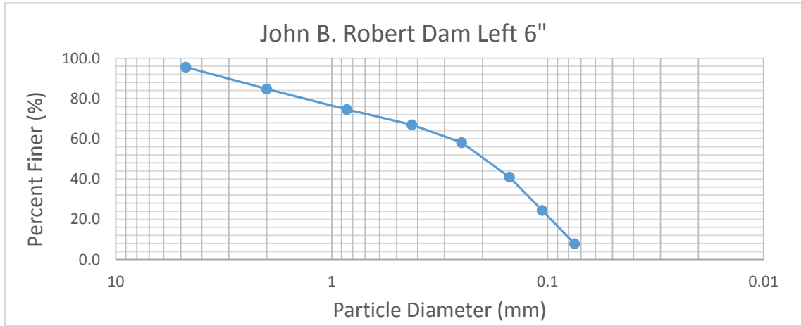
Figure 39: 6" Left Location - Sieve Analysis JBR Dam
